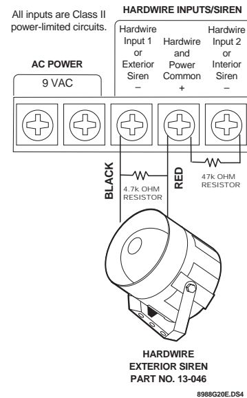
Figure 3. Supervised Exterior Siren Connections
