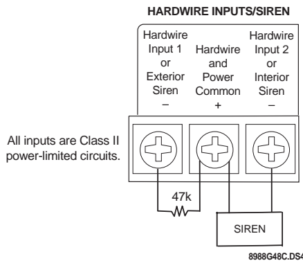
Figure 2. Supervised Interior Siren Connections
